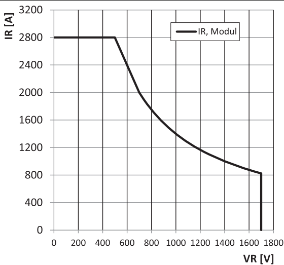
Fig. 11: SOA Diode
