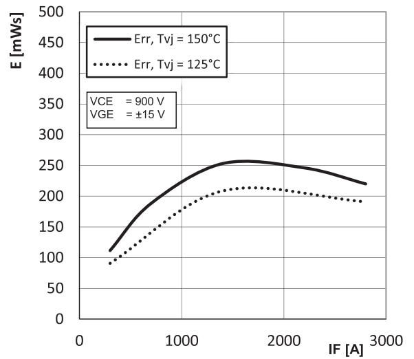
Fig. 8: Switching losses Diode (typical) E=f(I_F)
